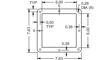
6 x 6 Top and Bottom Flange D35
